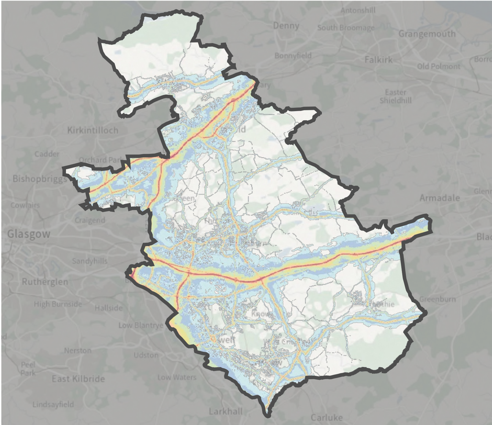
Figure 9.2 Round 4 Road Traffic Noise Levels L_{night}
