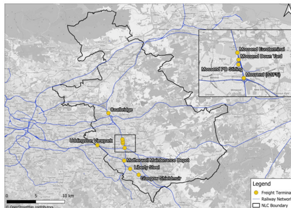
Figure 32: North Lanarkshire Rail Freight Terminals
